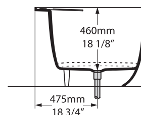
Section BB Shown with K12 waste kit
