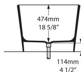
Section BB Shown with K12 waste kit
